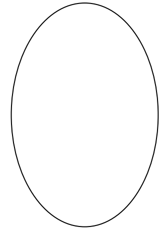
ovale
