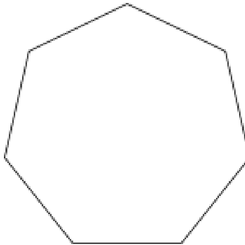
heptagone
