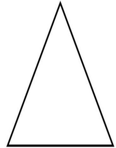
triangle acutangle
