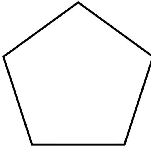
pentagone
