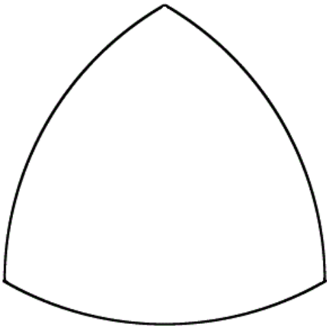
triangle curviligne
