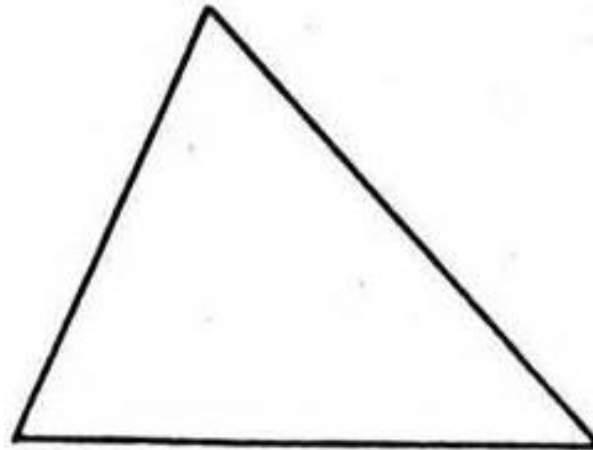
triangle scalène
