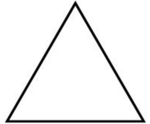
triangle
