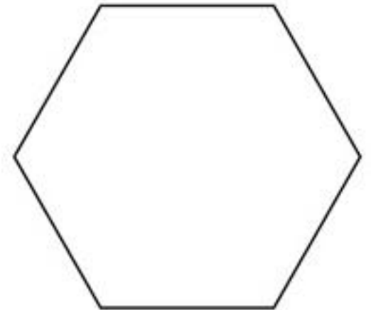
hexagone
