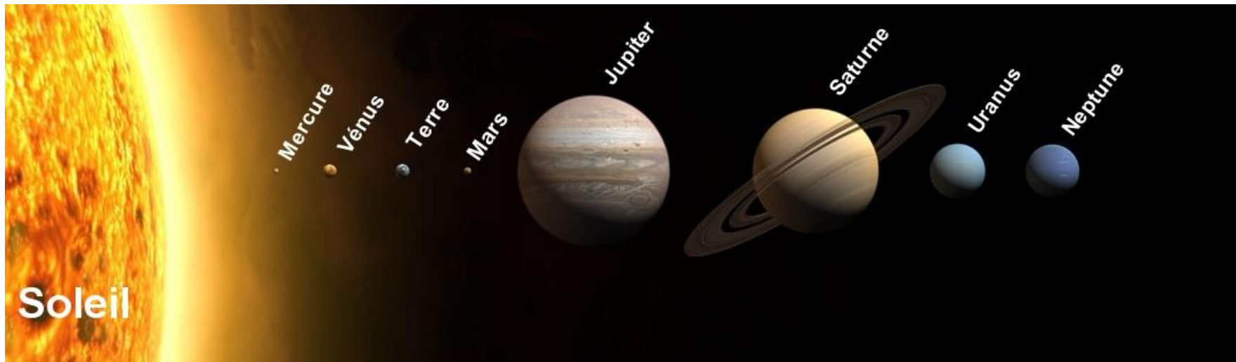
Neptune
