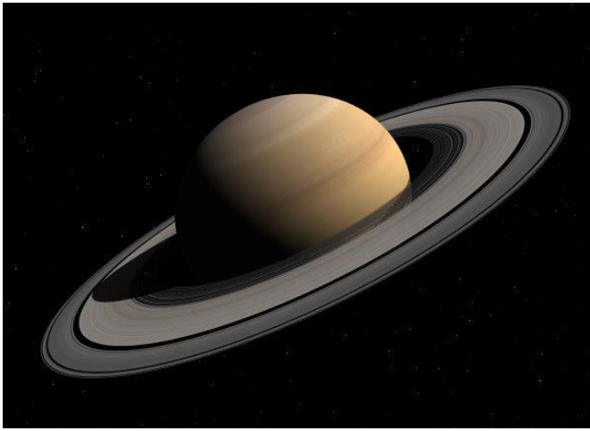
Saturne
