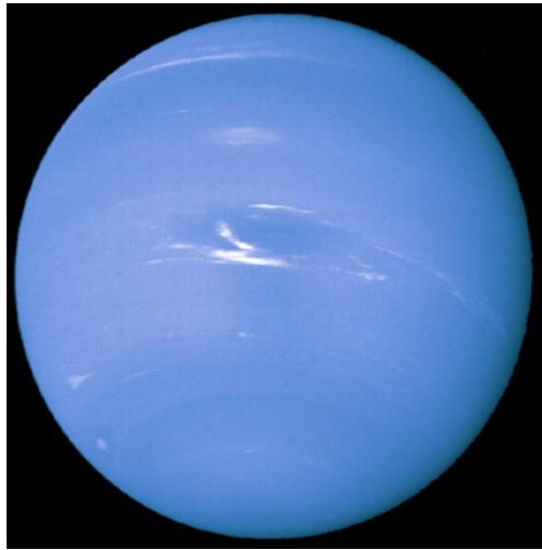
Neptune
