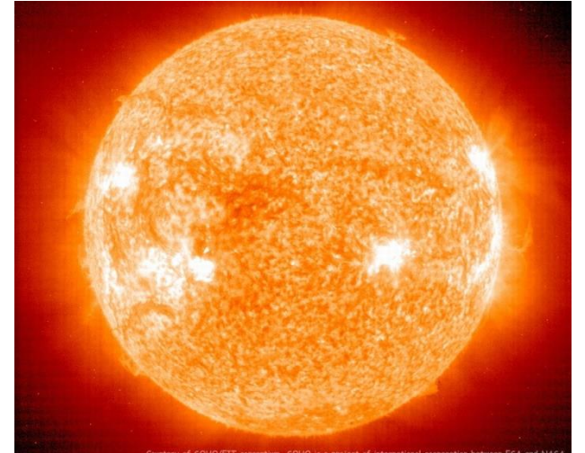
Soleil
